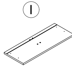
I DRAWER FRONT T7533196091GO QTY: 1 PC
